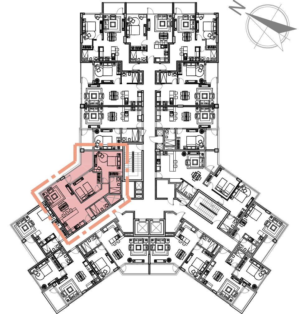
KEY PLAN
